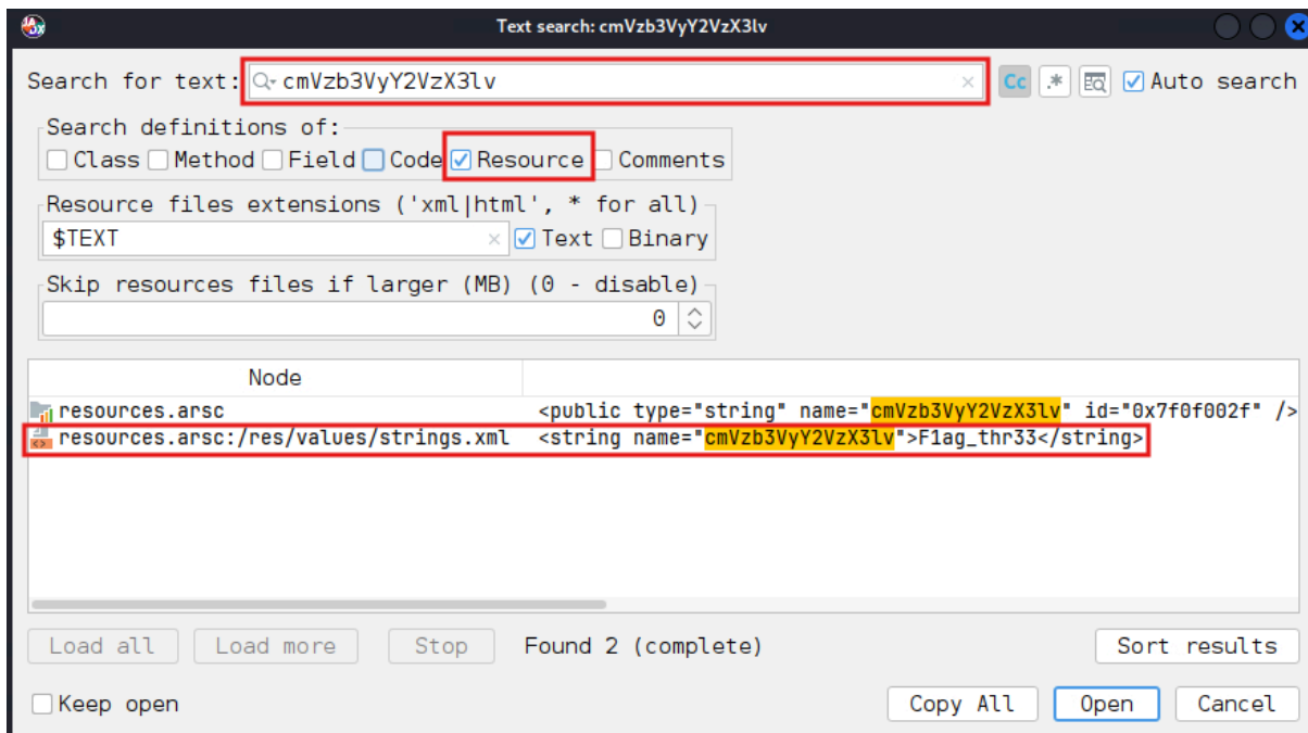
Figure 3: Displays Successful Search Result Found the Stored String Named "cmVzb3VyY2VzX3lv"
